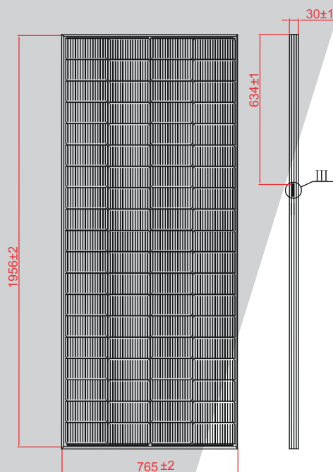
▼ Engineering Drawings (Front Side)
