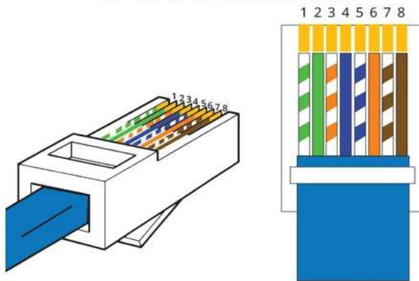
RJ-45 CAN BUS PINOUT
